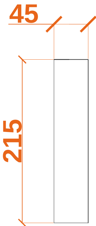
Side Elevation
