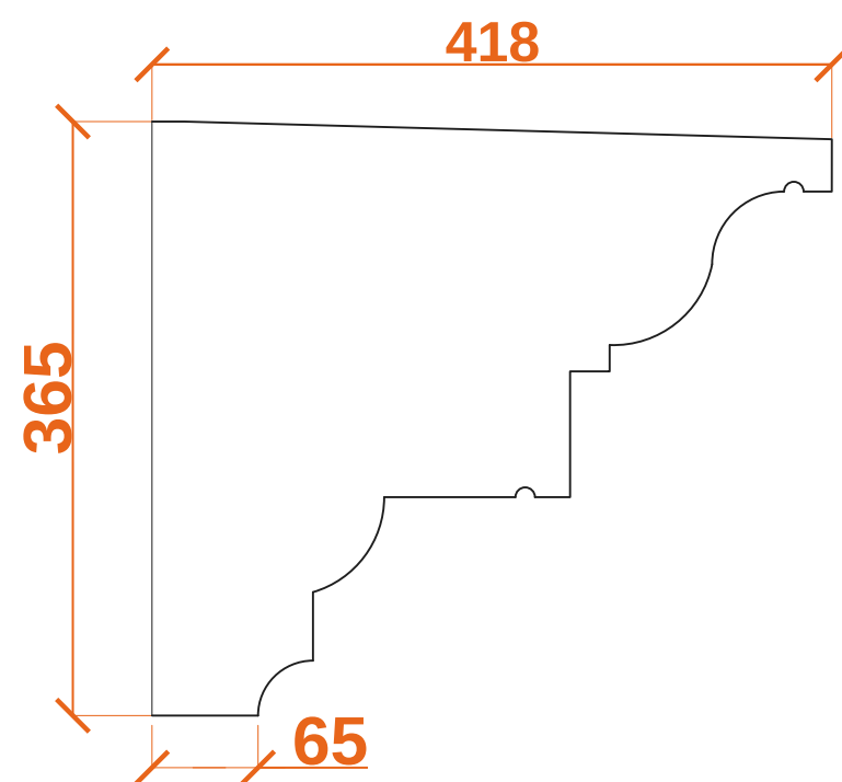
Side Elevation
